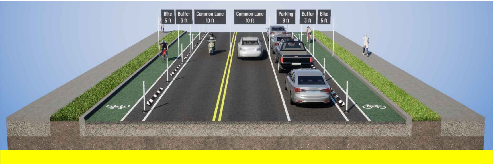
TYPICAL SECTION: LONG BLVD FROM ACKLEN PARK DRIVE TO BURNS AVE
